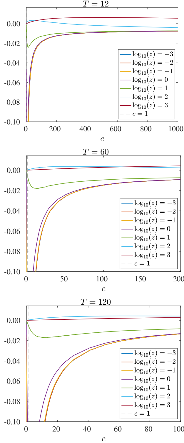
Figure IA3: Out-of-sample R^2 detail.
