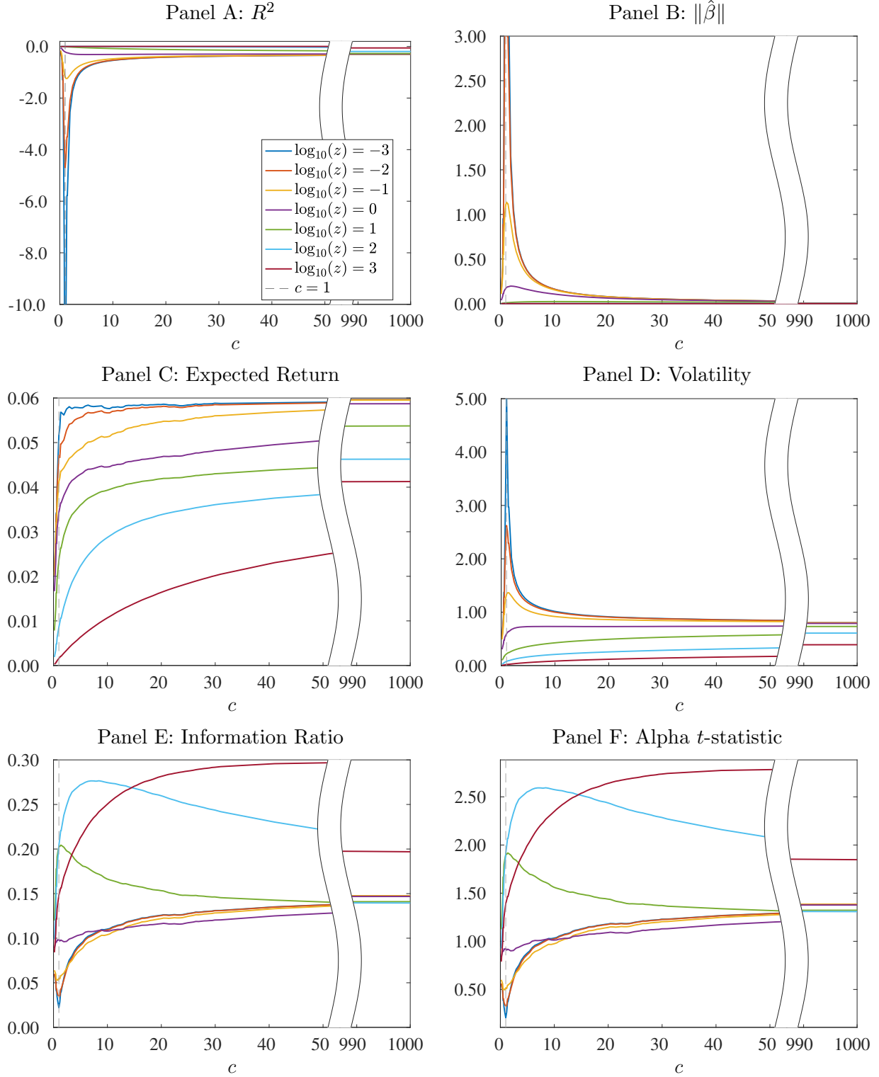
Figure IA7: Out-of-sample market timing performance with bandwidth \gamma = 1 .
