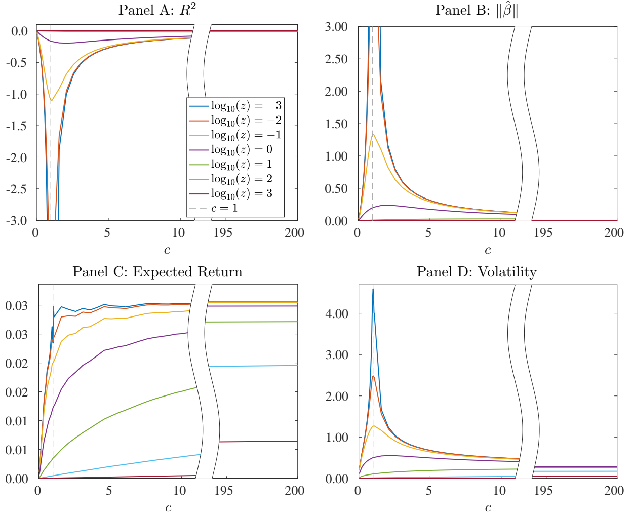
Figure IA1: Out-of-sample market timing performance with 60-month training window.
