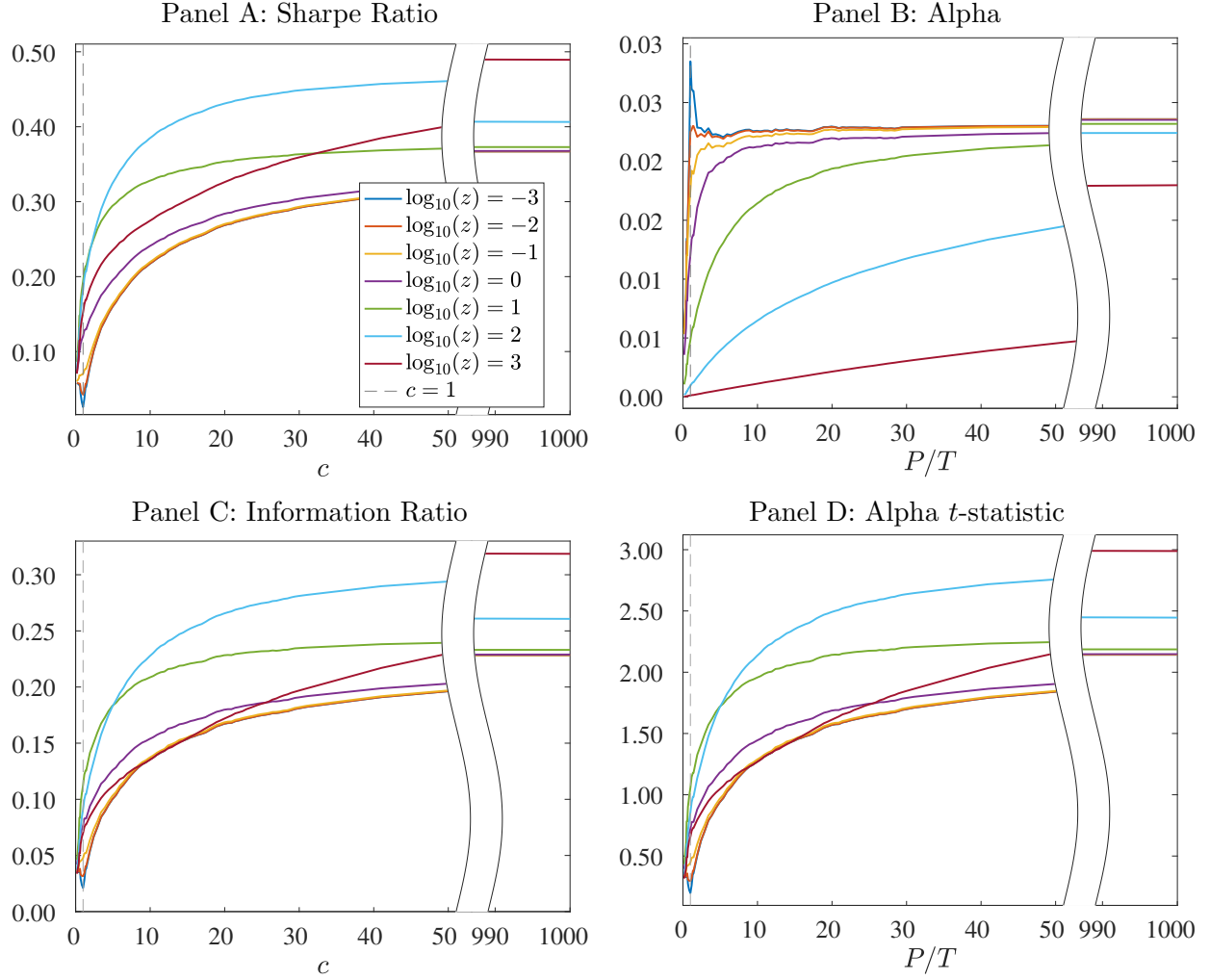
Figure IA12: Out-of-sample market timing performance with inflation excluded ( T = 12 ).
