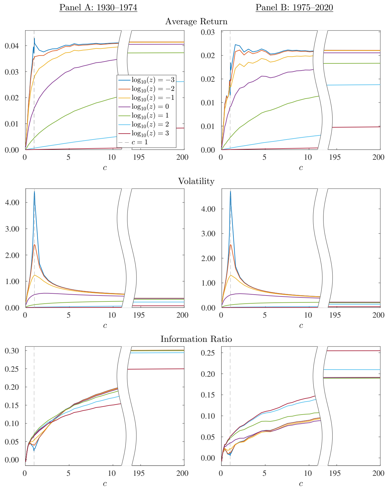
Figure IA10: Out-of-sample performance by subsample for ( T = 60 ).
