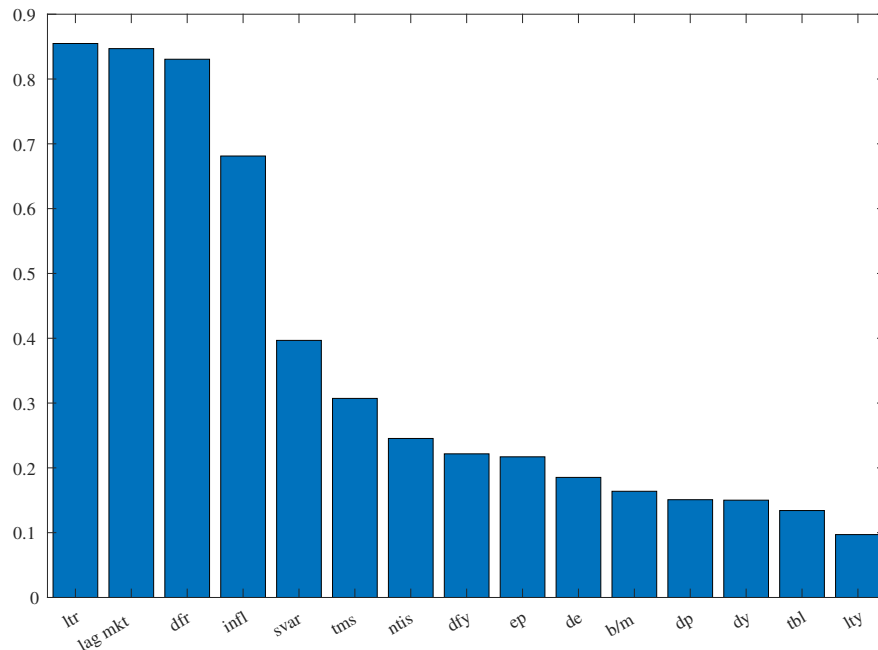
Figure IA4: Normalized volatility of predictors in 12-month windows.
