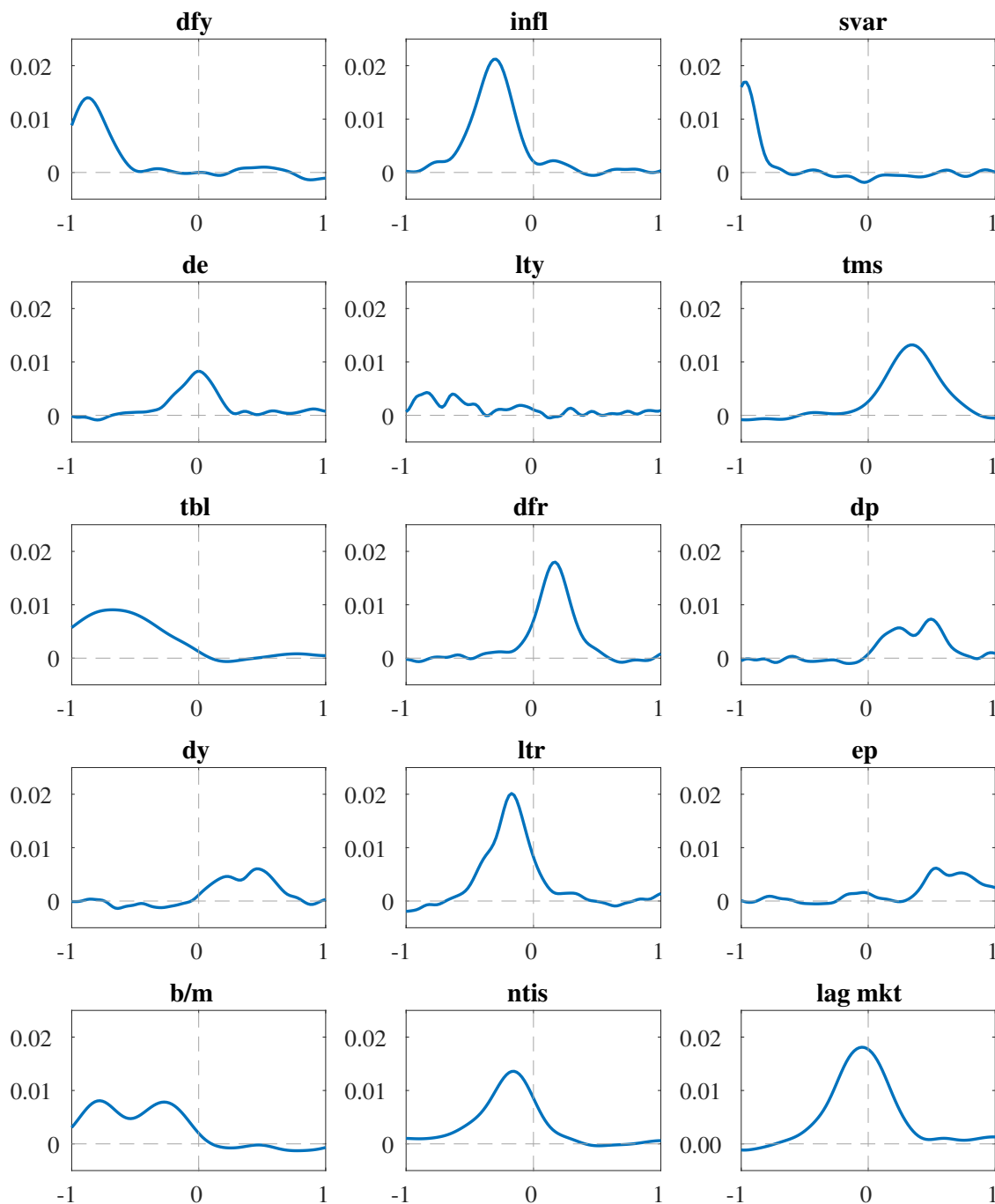
Figure IA5: Nonlinear prediction effects.
