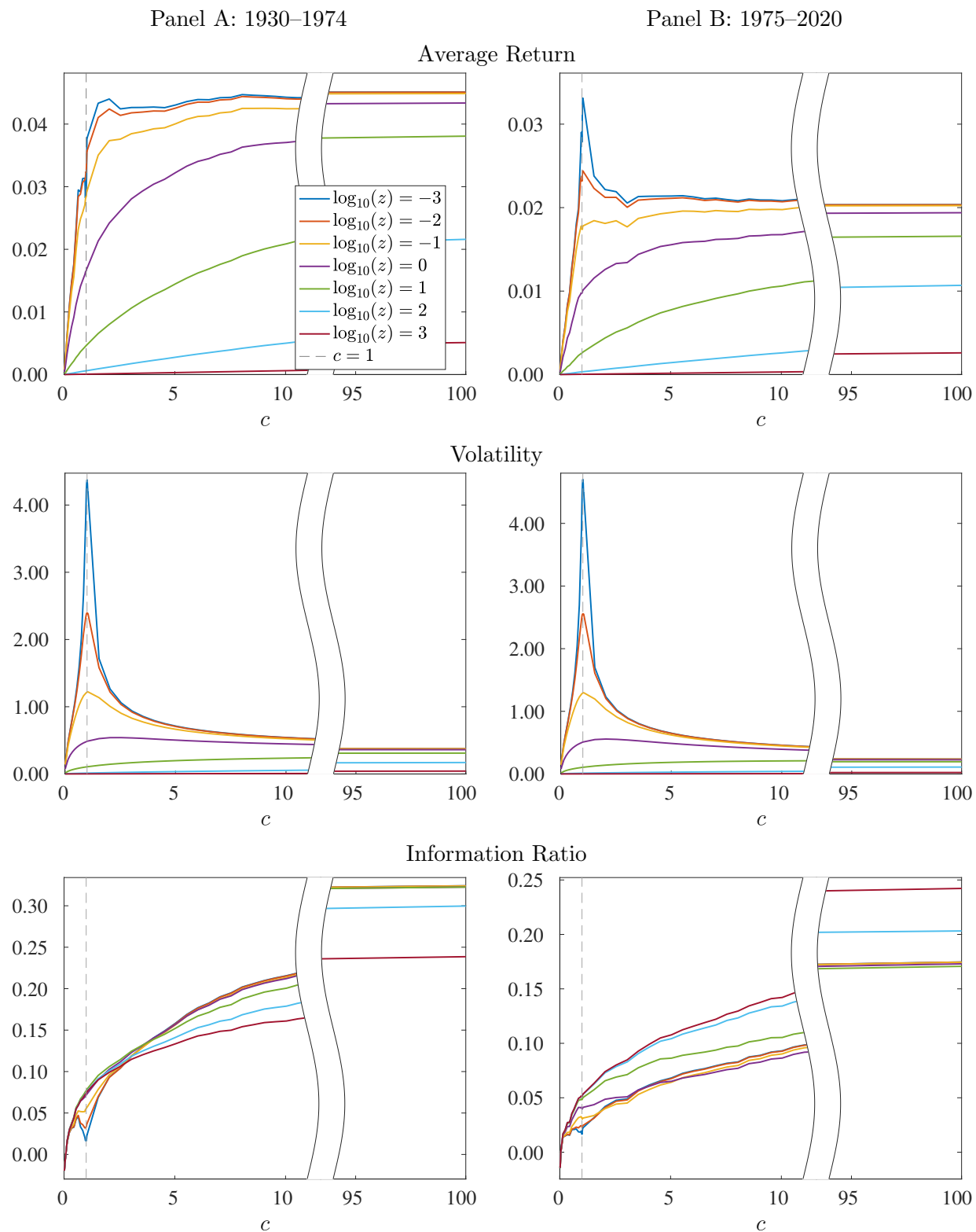
Figure IA11: Out-of-sample performance by subsample for ( T = 120 ).
