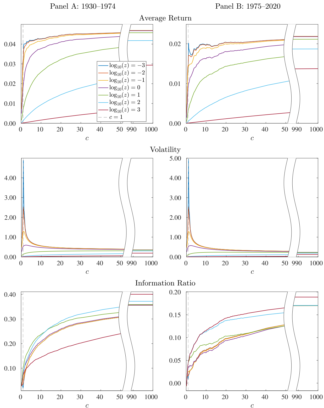
Figure IA9: Out-of-sample performance by subsample ( T = 12 ).
