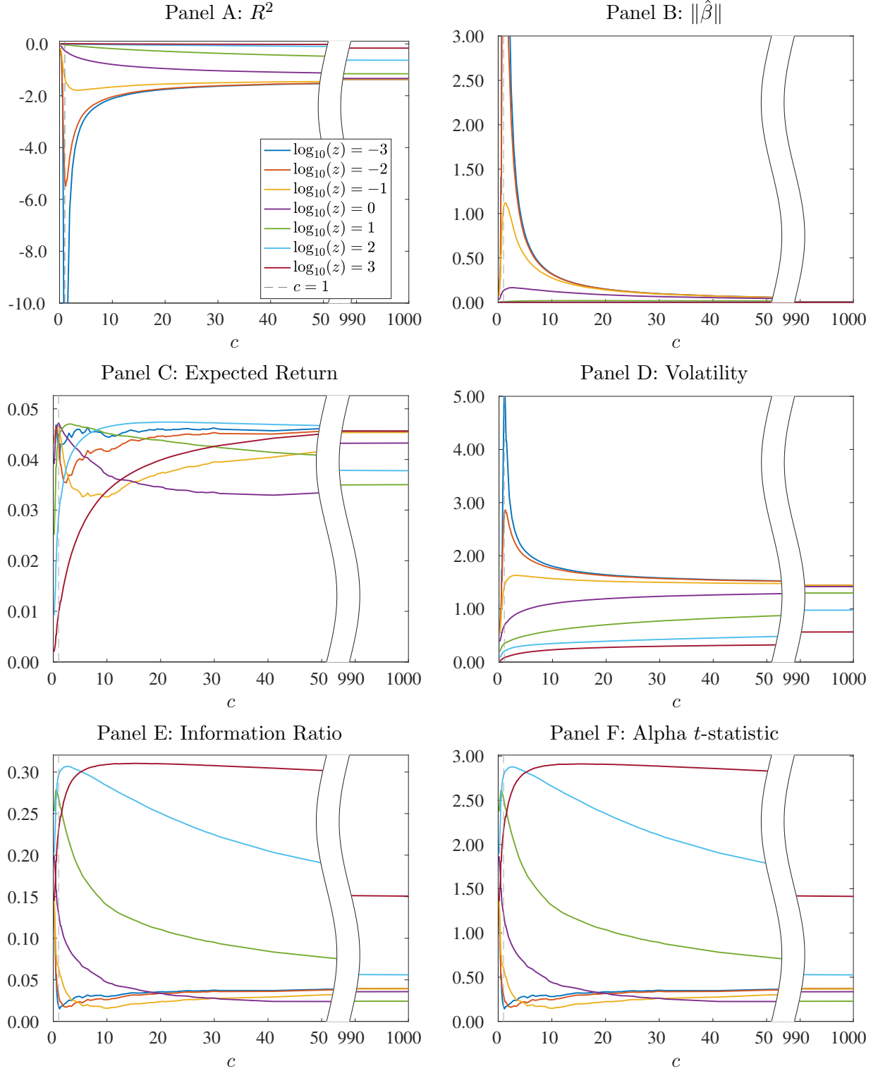
Figure IA8: Out-of-sample market timing performance with bandwidth \gamma = 0.5 .
