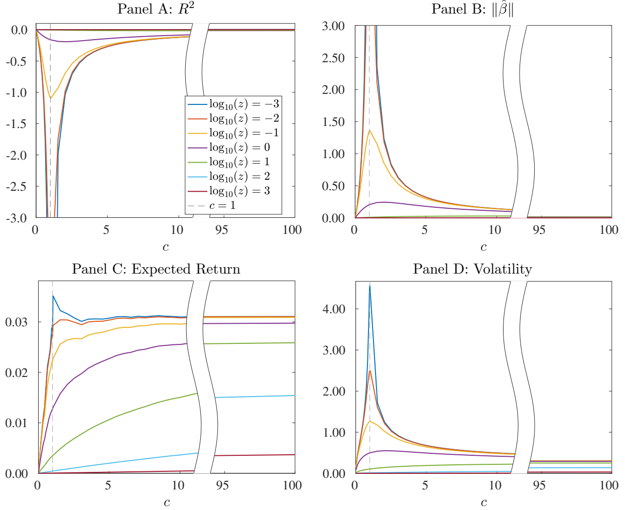
Figure IA2: Out-of-sample market timing performance with 120-month training window.
