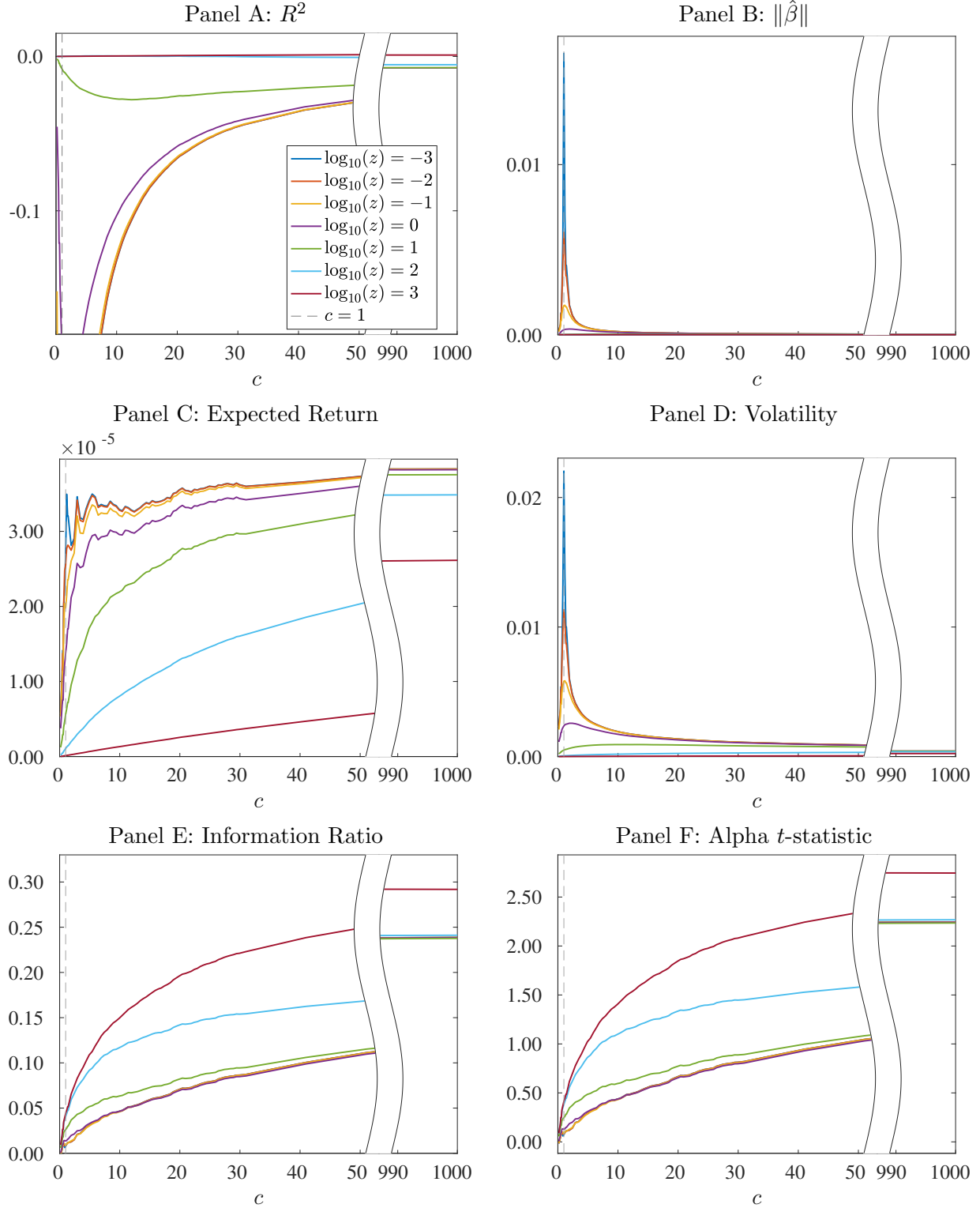
Figure IA6: Out-of-sample market timing performance with un-standardized returns.
